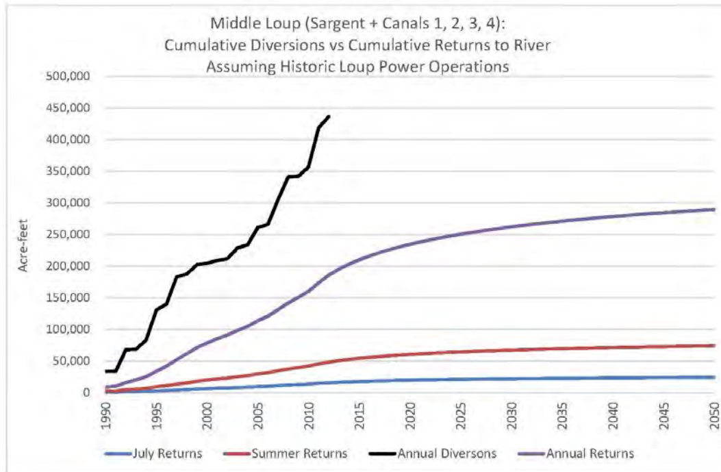
Figure 68: Cumulative Middle Loup Canal Diversions versus Cumulative Returns to Middle Loup River (assuming historic Loup Power Canal diversion)
