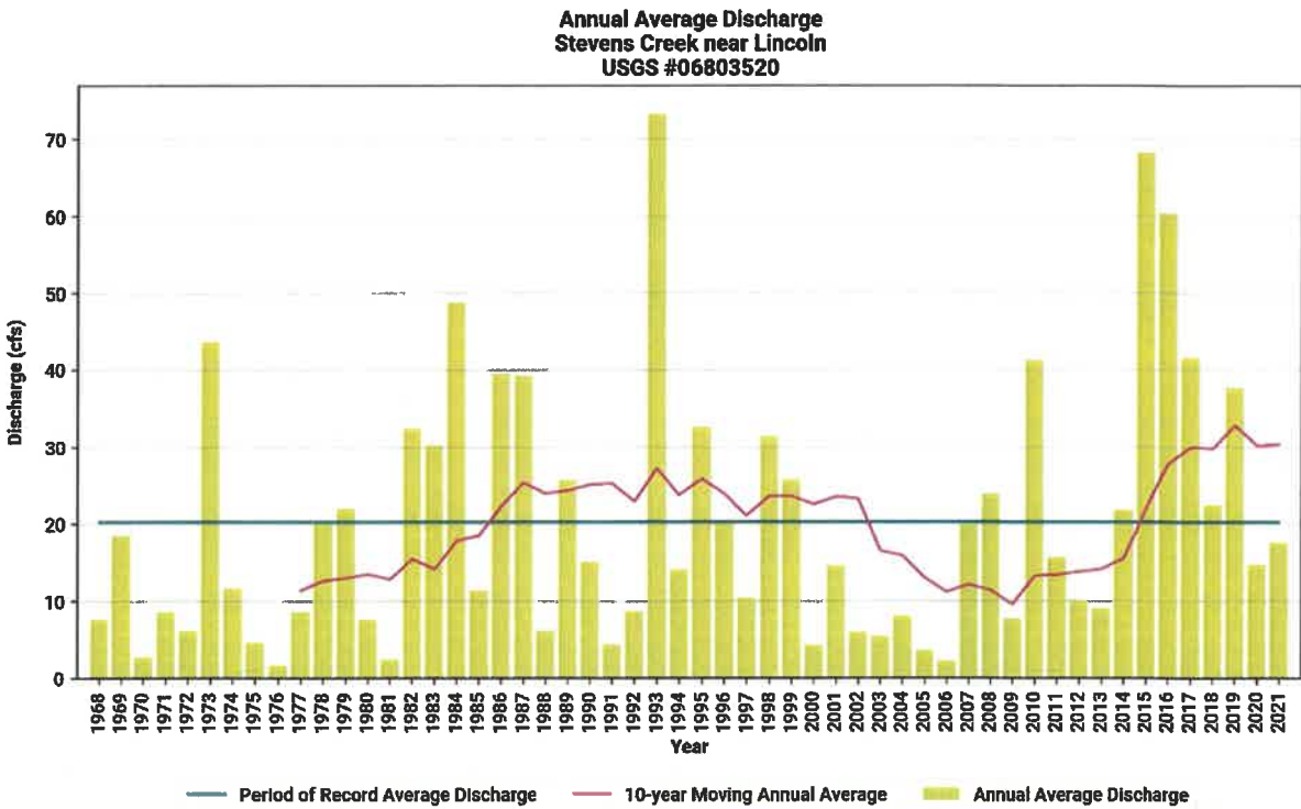
Figure 5: Historical annual discharge for Stevens Creek near Lincoln, NE (USGS-NWIS).
