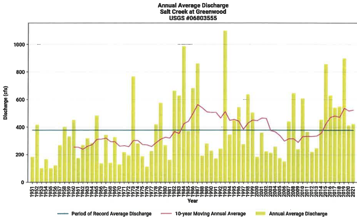
Figure 3: Historical annual discharge for Salt Creek at Greenwood, NE (USGS-NWIS).
