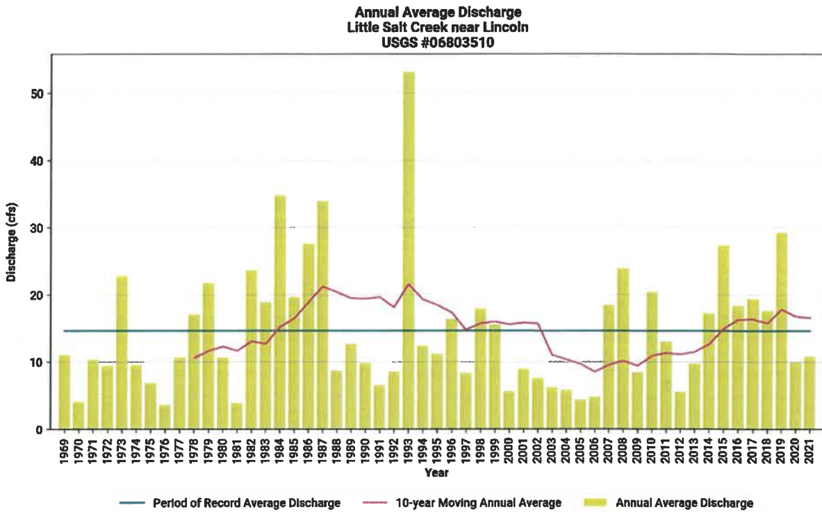
Figure 4: Historical annual discharge at Little Salt Creek near Lincoln, NE (USGS-NWIS).
