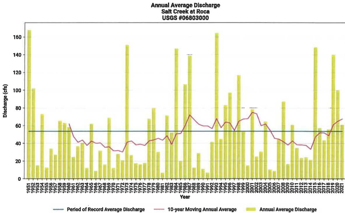
Figure 2: Historical annual discharge for Salt Creek at Roca, NE (USGS-NWIS).
